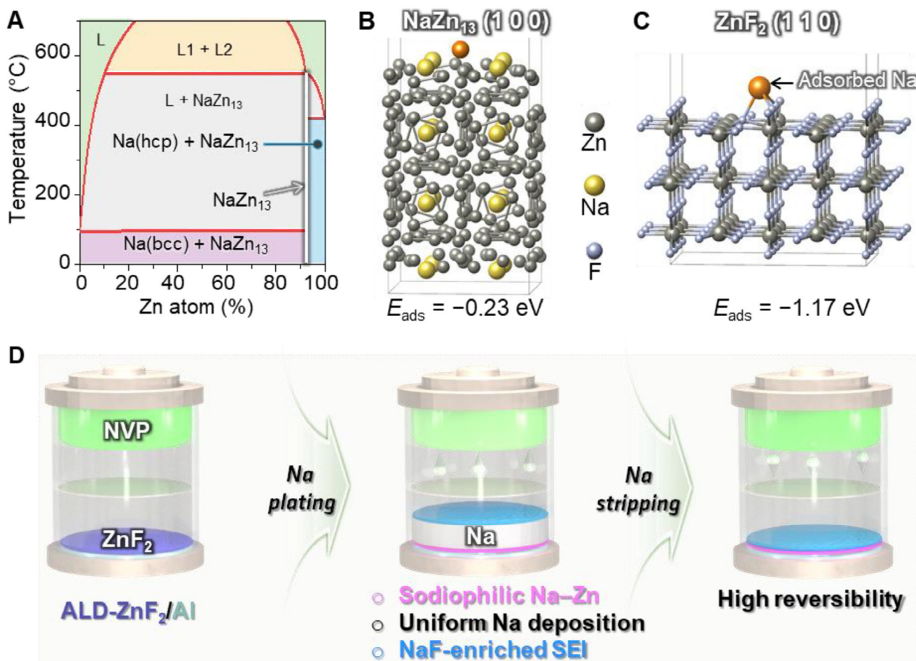
FIGURE 1 | Schematic design of the ZnF 2 /Al host for stable AFSBs. (A) Na–Zn phase diagram [29]. (B,C) DFT-optimized configurations and adsorption energies of Na on NaZn 13 (100) and ZnF 2 (110) surfaces, respectively. (D) AFSB configuration using ZnF 2 /Al as the current collector. An ultrathin ZnF 2 layer deposited by ALD is converted during the first Na plating (sodiation) into a NaF/Na–Zn interphase; the sodiophilic Na–Zn promotes uniform Na nucleation and growth, while the NaF-enriched SEI stabilizes the interface, enabling dense Na deposits and highly reversible cycling.
