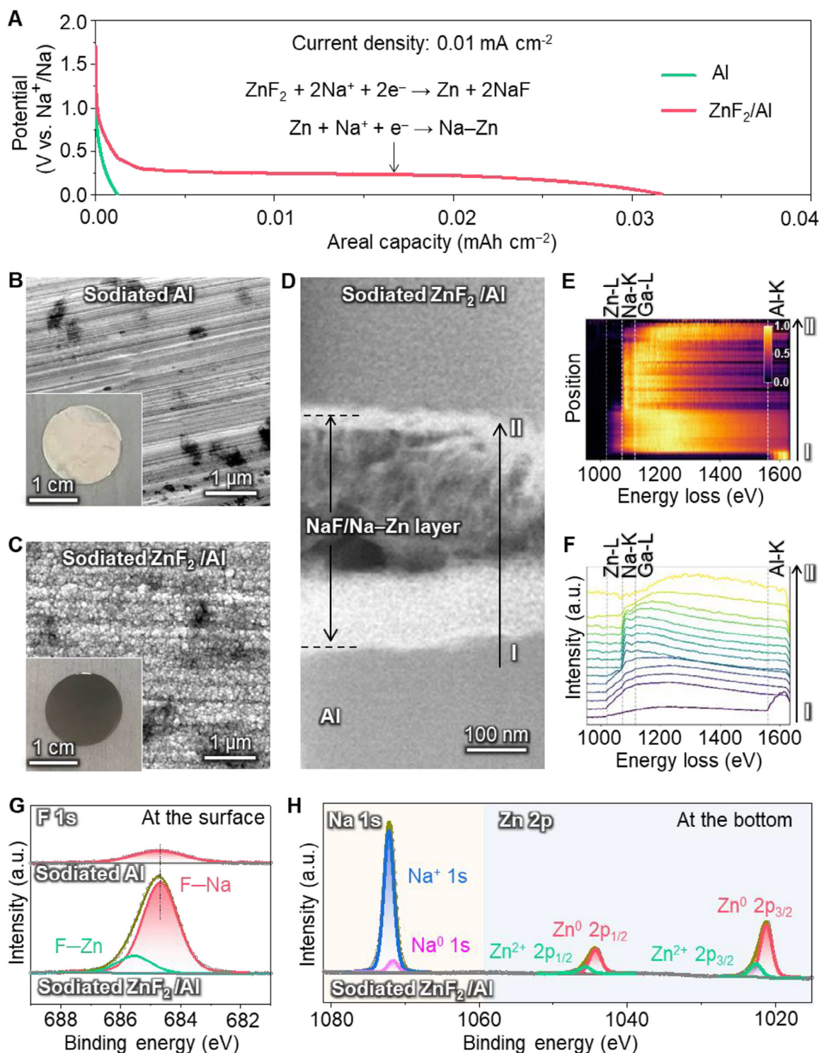
FIGURE 3 | Electrochemical activation of the ALD-ZnF 2 layer and formation of the NaF/Na-Zn interphase. (A) First-discharge profiles of Na||Al and Na||ZnF 2 /Al cells. (B,C) SEM images of sodiated Al and sodiated ZnF 2 /Al current collectors (insets: optical photographs). (D) Cross-sectional ADF-STEM image of sodiated ZnF 2 /Al. (E) 2D EELS intensity map acquired along the line from point I to point II, showing the spatial distribution of core-loss edges across the reaction layer. (F) EELS line-profile spectra (5-spectrum binned averages with LOESS smoothing). Dashed lines indicate the onset energies of Zn L 3 (~1020 eV), Na K (~1072 eV), Ga L 3 (~1115 eV, FIB artifact), and Al K (~1560 eV). (G,H) Fitted XPS spectra of F 1s at the surface of the NaF/Na-Zn layer and both Na 1s and Zn 2p at the bottom of the NaF/Na-Zn layer.
