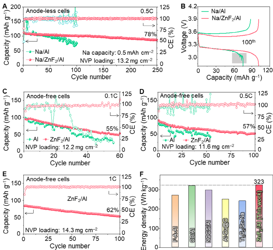
FIGURE 6 | Full-cell performance of ZnF 2 /Al current collectors in lean-Na and anode-free configurations. (A) Cycling performance of Na/Al || NVP and Na/ZnF 2 /Al || NVP lean-Na cells with a low N/P ratio at 0.5 C. (B) Charge-discharge voltage profiles of Na/Al || NVP and Na/ZnF 2 /Al || NVP cells at the 100th cycle. The grey region highlights irregular voltage fluctuations of the Na/Al || NVP cell. (C–E) Cycling performance of Al || NVP and ZnF 2 /Al || NVP anode-free cells at 0.1C (C), 0.5C (D), and 1C (E). (F) Comparison of the energy densities of AFSBs calculated based on the total mass of positive and negative electrode active materials, using different anode-side hosts: fluorinated Al (F-A-Al) [9], carbon-black-coated Al (CB/Al) [44], N, O-co-doped carbon-sphere-coated Al (NOCS/Al) [45], Cu-C-coated Al (Al-Cu@C) [46], MXene/Tin-Na (Ti 3 C 2 /Sn-Na) [47], and the present ZnF 2 /Al.
