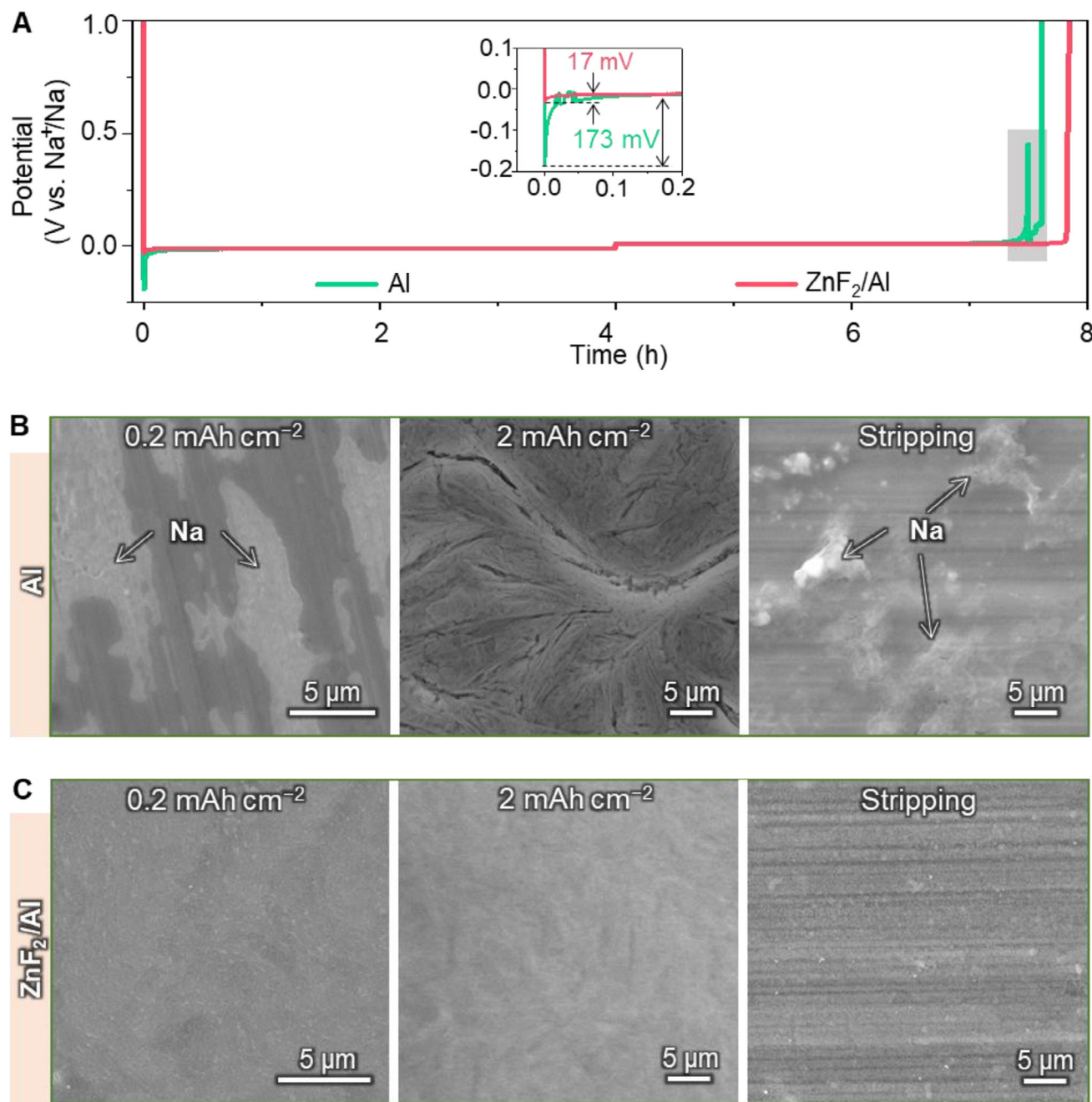
FIGURE 4 | Effect of the NaF/Na-Zn interphase on Na plating/stripping behavior. (A) Voltage profiles of Na plating/stripping on bare Al and ZnF 2 /Al at 0.5 mA cm -2 . The inset shows the Na nucleation overpotentials. The grey region highlights irregular voltage fluctuations of the Na||Al cell. (B) SEM images of Na deposited on bare Al at 0.2 and 2.0 mAh cm -2 , and after subsequent stripping. (C) Corresponding SEM images for ZnF 2 /Al.
