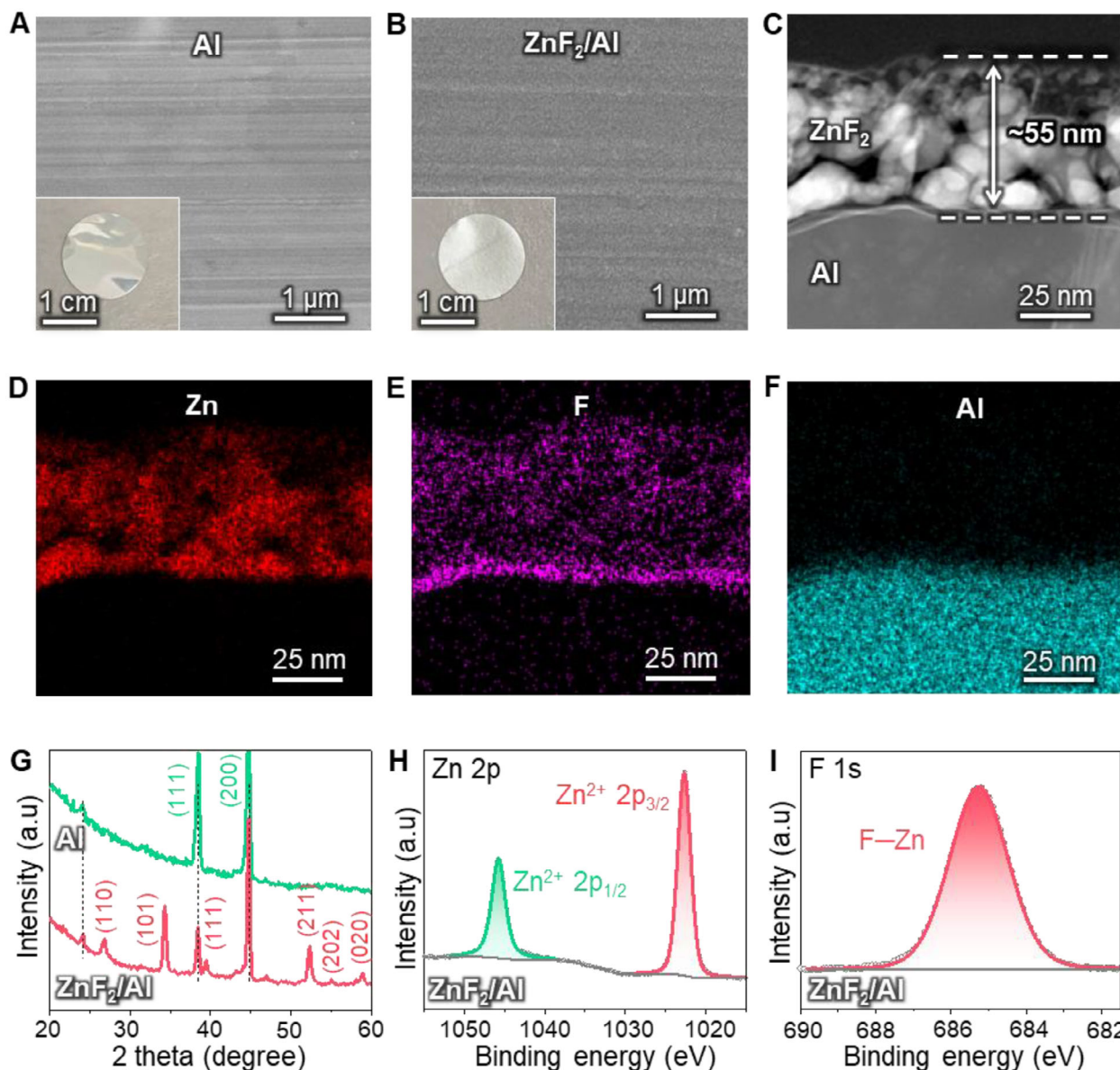
FIGURE 2 | Structural and chemical characterization of the ALD-ZnF 2 coating on Al foil. (A,B) SEM images of bare Al and ZnF 2 /Al CCs, respectively (insets: corresponding optical photographs). (C) Cross-sectional STEM-HAADF image showing an ultrathin ZnF 2 layer with a thickness of ~55 nm uniformly covering the Al substrate. (D,F) STEM-EDX elemental maps of Zn, F, and Al, respectively. (G) XRD patterns of bare Al and ZnF 2 /Al. (H,I) Fitted XPS spectra of Zn 2p and F 1s for ZnF 2 /Al.
